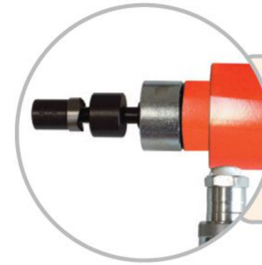
Punch cylinder assembly with dies and stud.
